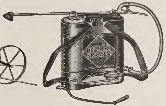
Hudson DU-MORE. For all purpose spraying. Continuous spray by a slow stroke of powerful diaphragm pump. 4 gal. capacity, 3 ft. hose, 2 ft. extension rod, shut-off valve and adjustable nozzle.
